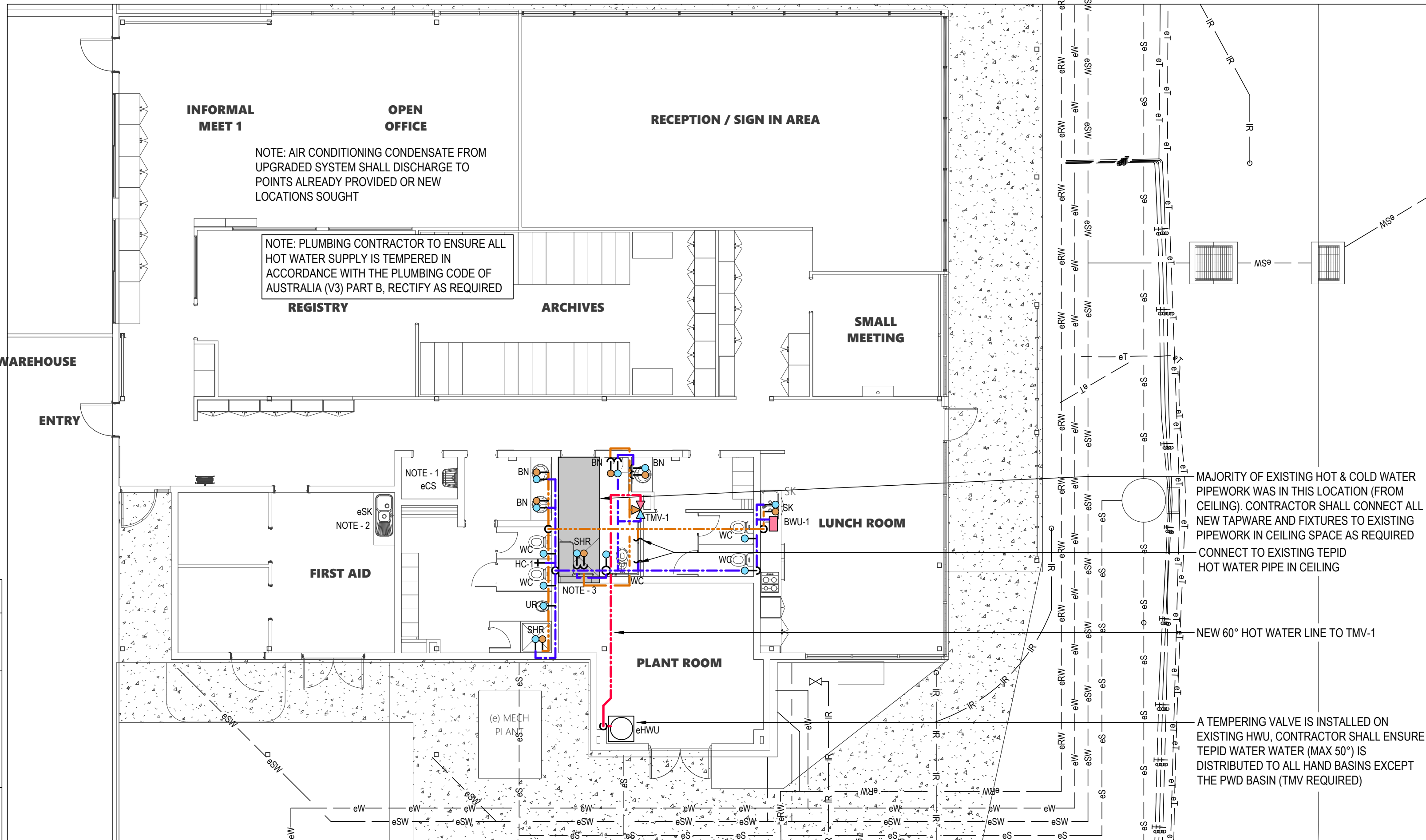
2 Proposed Floor Plan - Water
