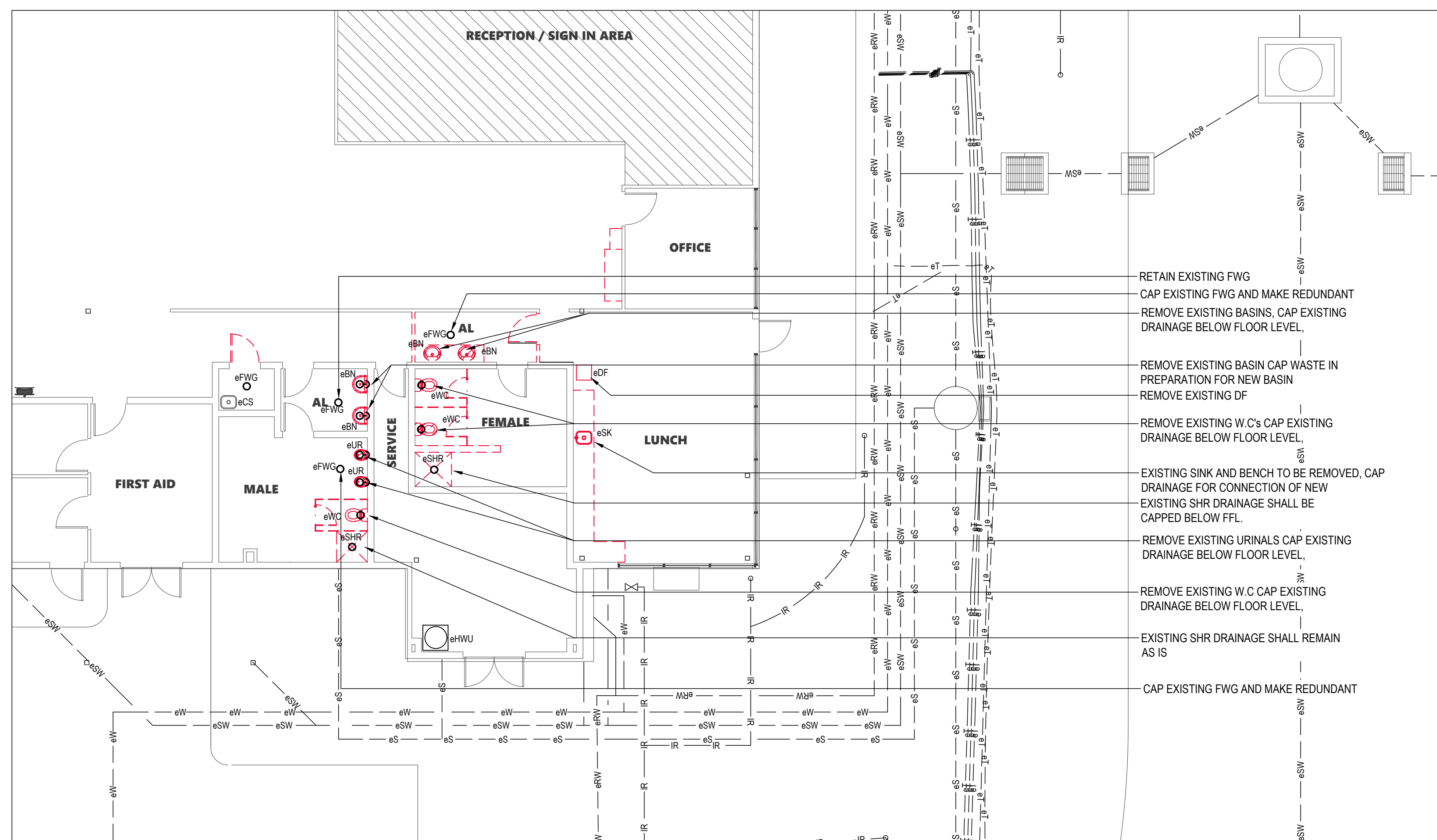
1 Existing Floor Plan - Drainage demolition
