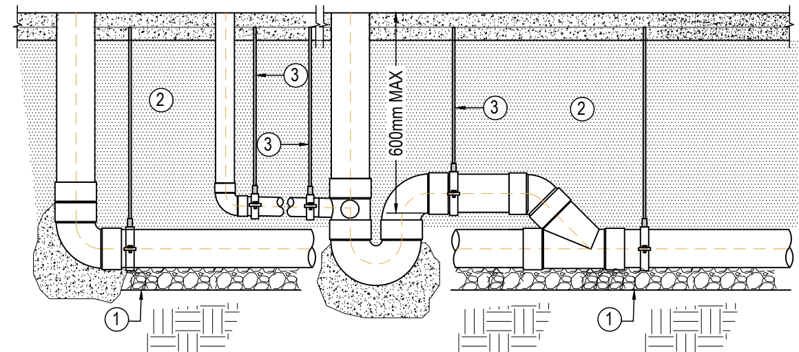
RECOMMENDED PIPE SUPPORT LOCATIONS ON "E" TYPE SOILS NOT TO SCALE
