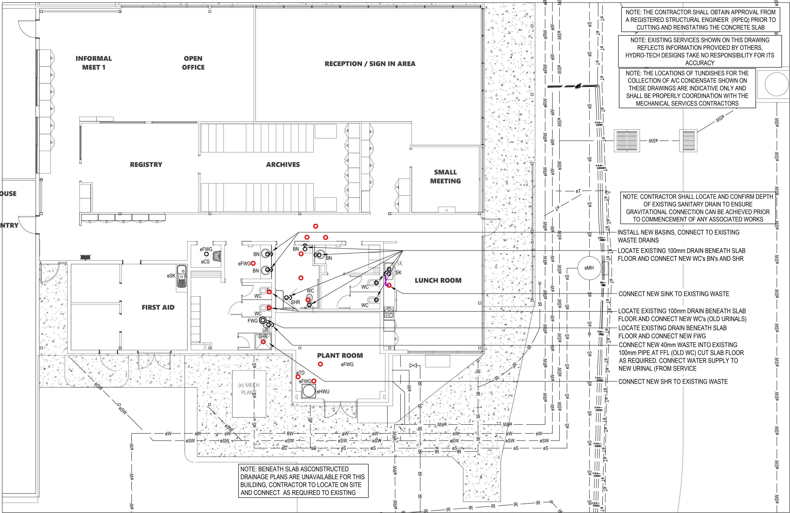
1 Proposed Floor Plan - Drainage
