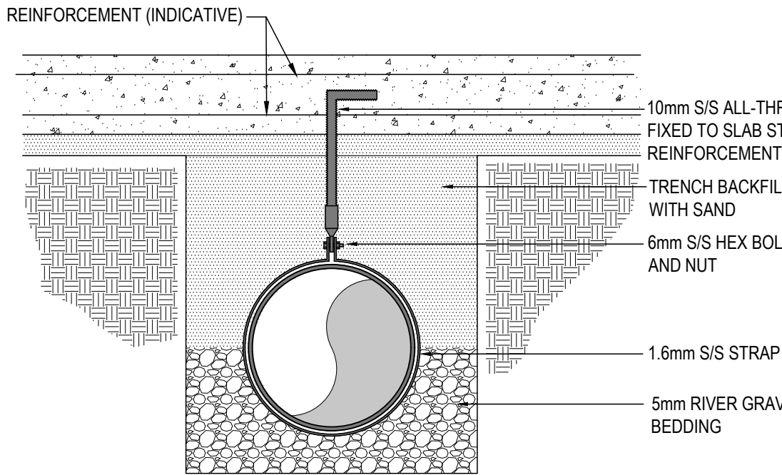
DETAIL - 'A': SUPPORT BRACKET FOR DRAINS BENEATH BUILDING FLOOR NOT TO SCALE
