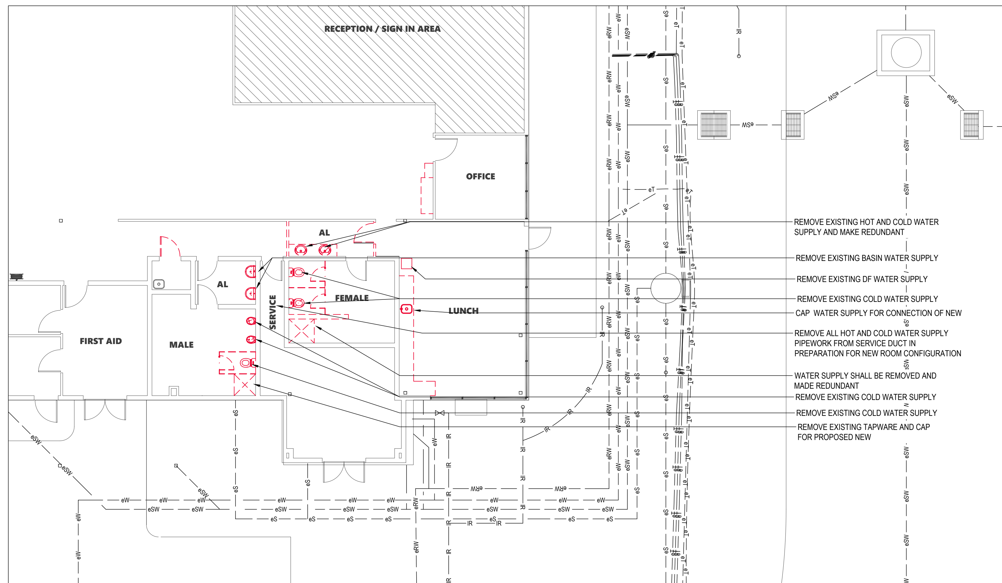
2 Existing Floor Plan - Water demolition
